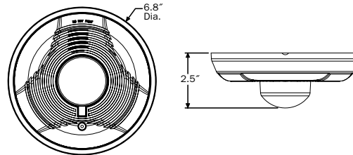
Ceiling-mount horn/strobes
